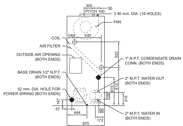
RIGHT END VIEW
