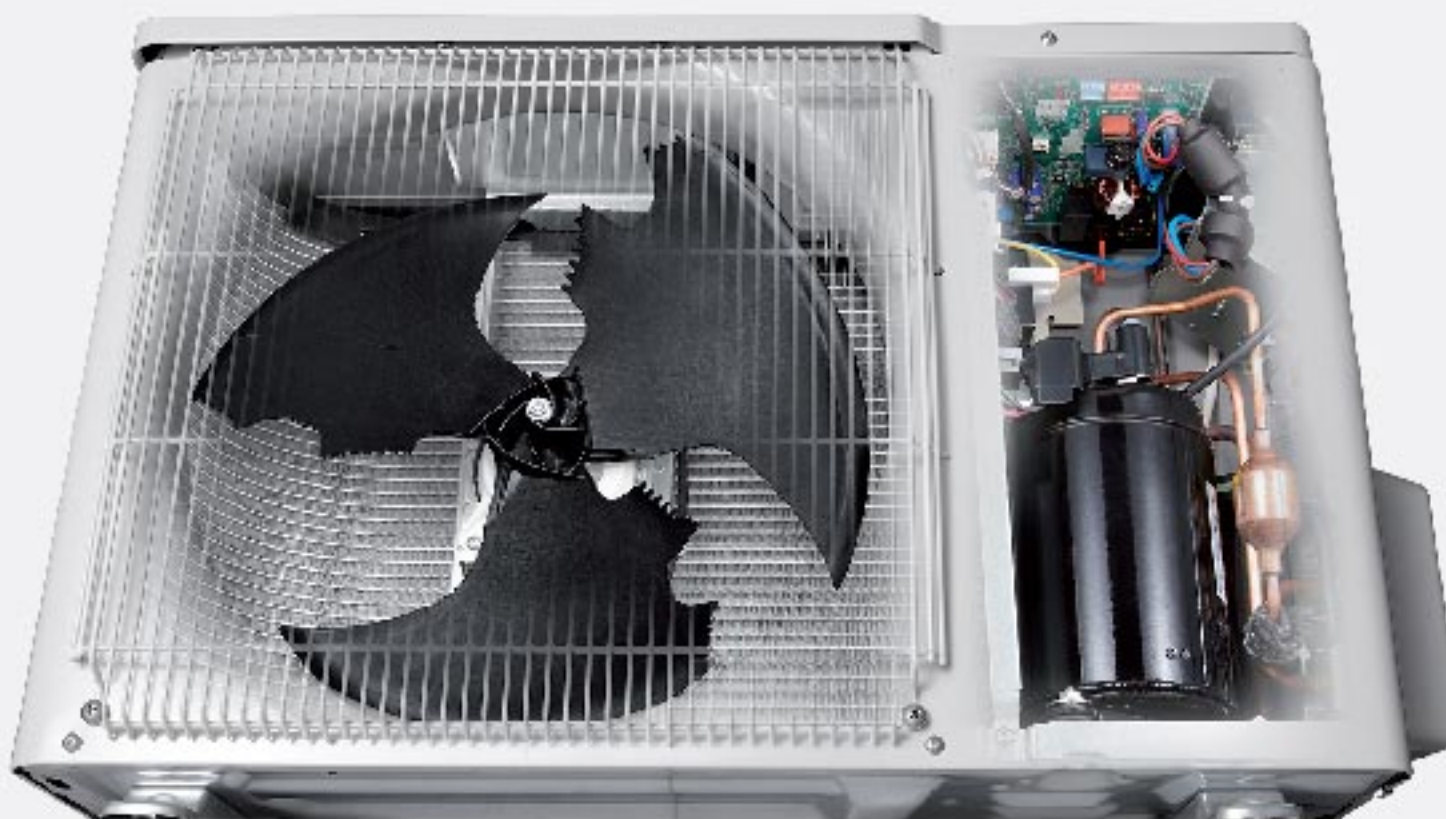
Multiflow Condenser
