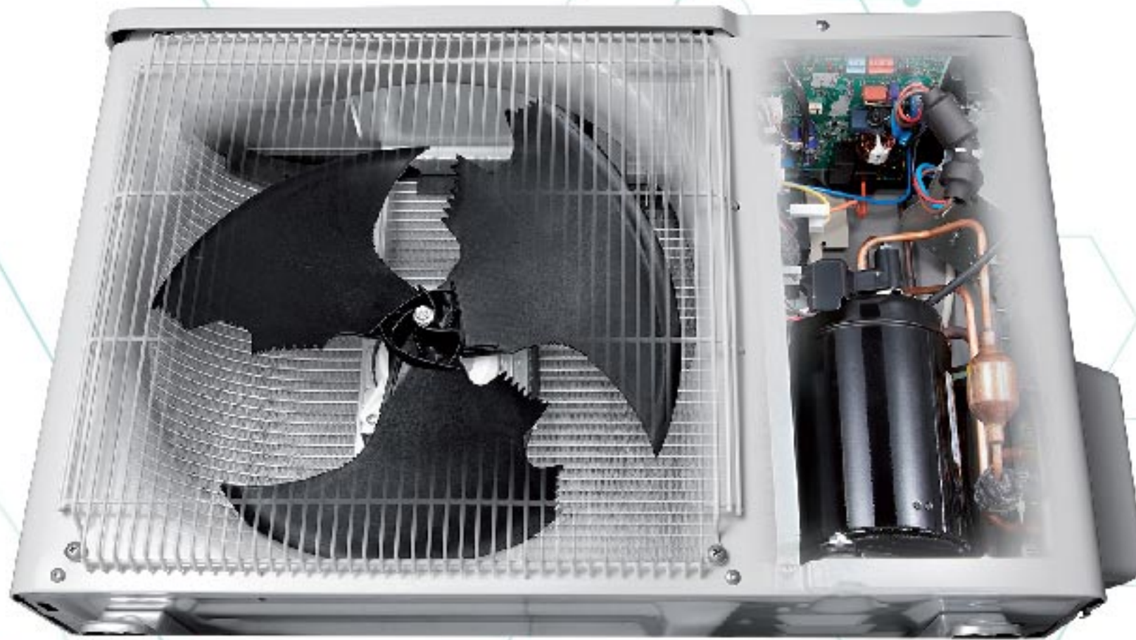
Multiflow Condenser
